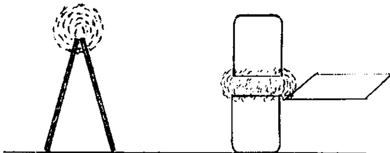
22-rasm. Oq tutunning hosil bo'lishi
