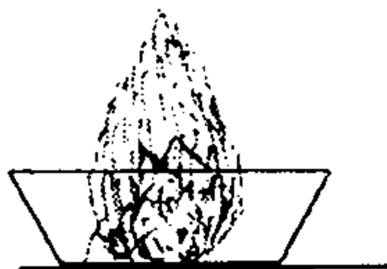
16-rasm. Qog'ozning yonishi.
