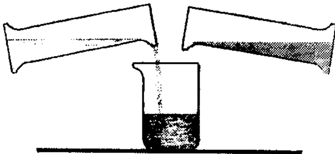
6-rasm. "Suv"ning "qon"ga aylanishi.
