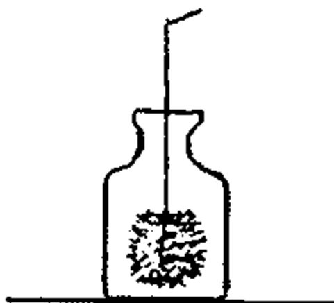
13-rasm. Temirning yonishi.
