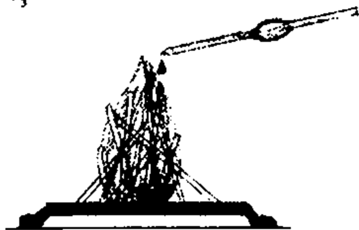
15-rasm. Gulxanning yonishi.
