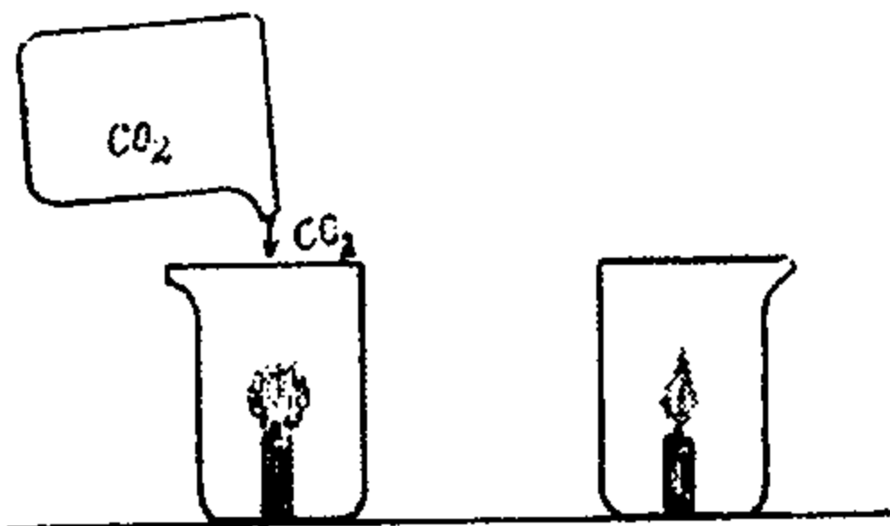
23-rasm. Shamlarning o'chishi.
