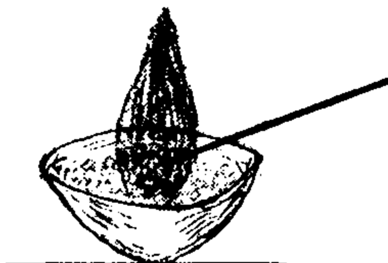
18-rasm. Qorning tutab “yonishi”
