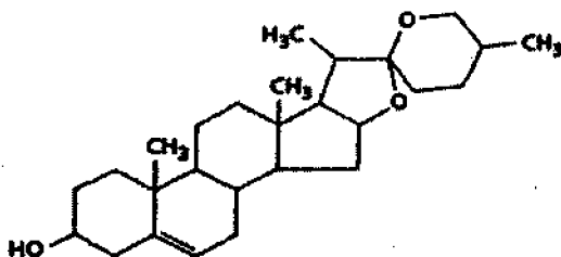
Yamogenin
