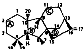
Ent-gibberellin
