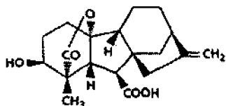
\Gamma A_4
