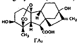
\Gamma A_1
