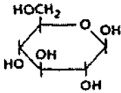
\beta -D-glyukoza
