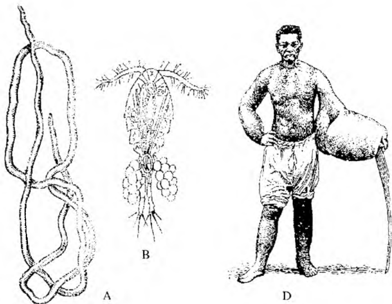
70-rasm. Parazit nematodalar.
