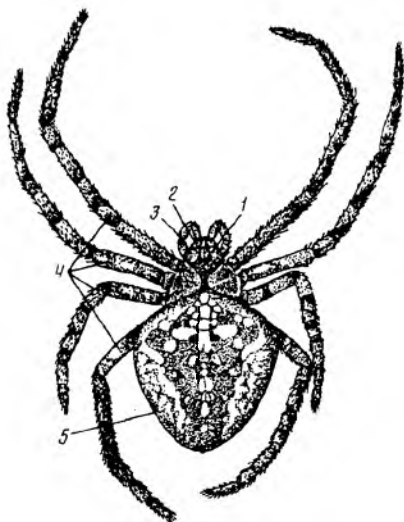
138-rasm. Butli o'rgimchak ( Araneus diadematus ).
