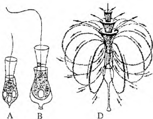
9-rasm. Yoqali xivchinlilar Choanoflagellata .
