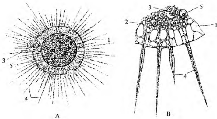
6-rasm. Chuchuk suv quyoshlisi ( Actinospaerium eichhorni ).
