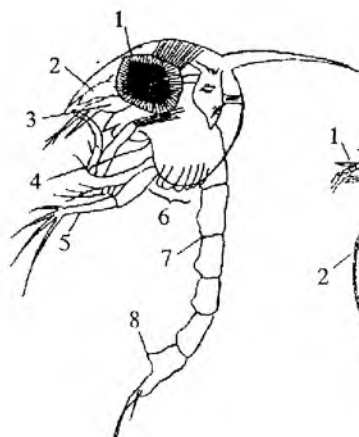
124-rasm. Krablarning zoyea lichinkasi.
