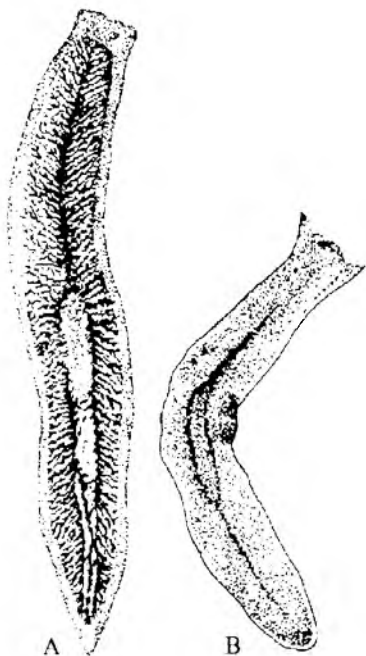
47-rasm. Kiprikli chualchaglar.
