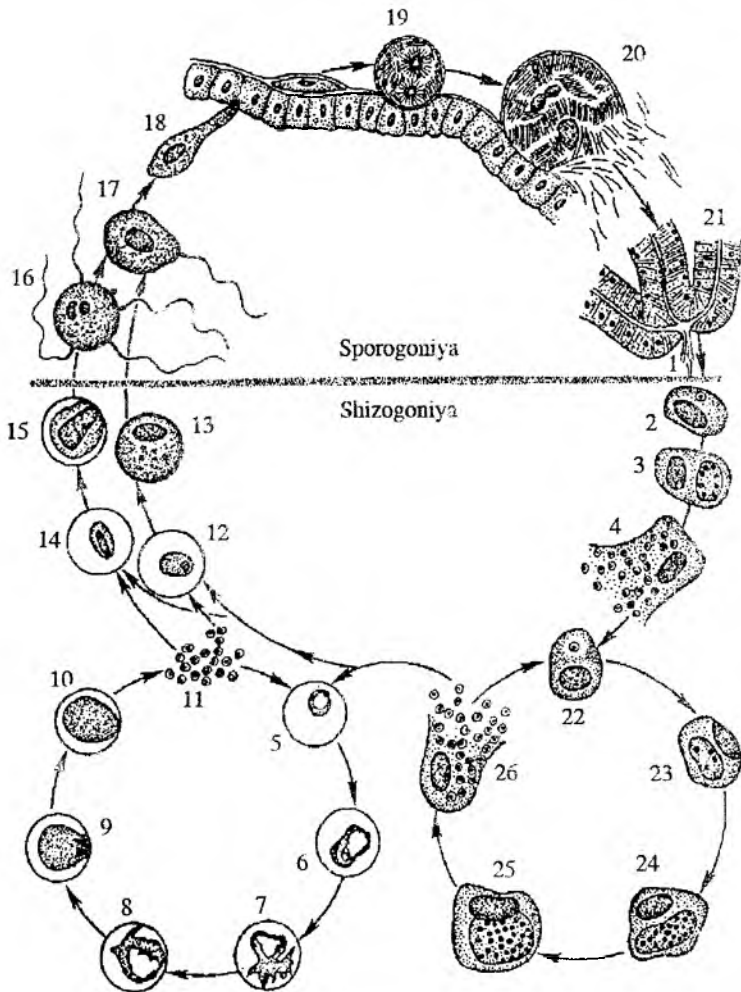
17-rasm. Bezagk parazitining hayot sikli.
