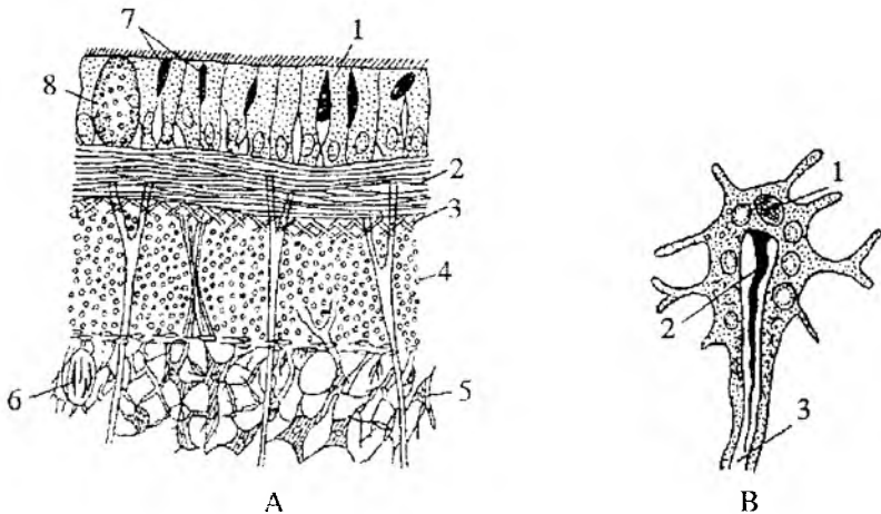
48-rasm. A – oq planariyaning teri-muskul xalta kesmasi: 1 – teri epiteliysi, 2 – halqali muskullar, 3 – qiyshiq muskullar, 4 – bo‘ylama muskullar, 5 – parenxima hujayralari, 6 – rabdit hosil qiluvchi hujayralar, 7 – rabditlar. 8 – teri bezlari. B– ayirish sistemasi uchki hujayrasi: 1 – yadro, 2 – xilpillovchi kipriklar, 3 – hujayra nayi.
