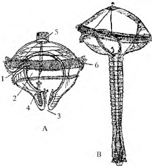
86-rasm. Troxofora (A) va uni voyaga yetgan chugalchangga (B) aylanishi.
