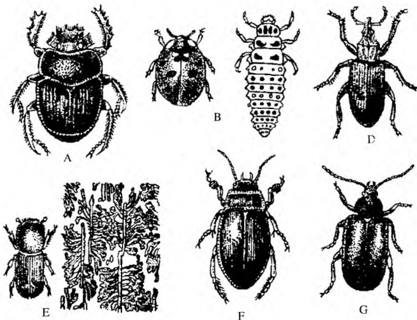
187-rasm. Qattiq qanotlilar.
