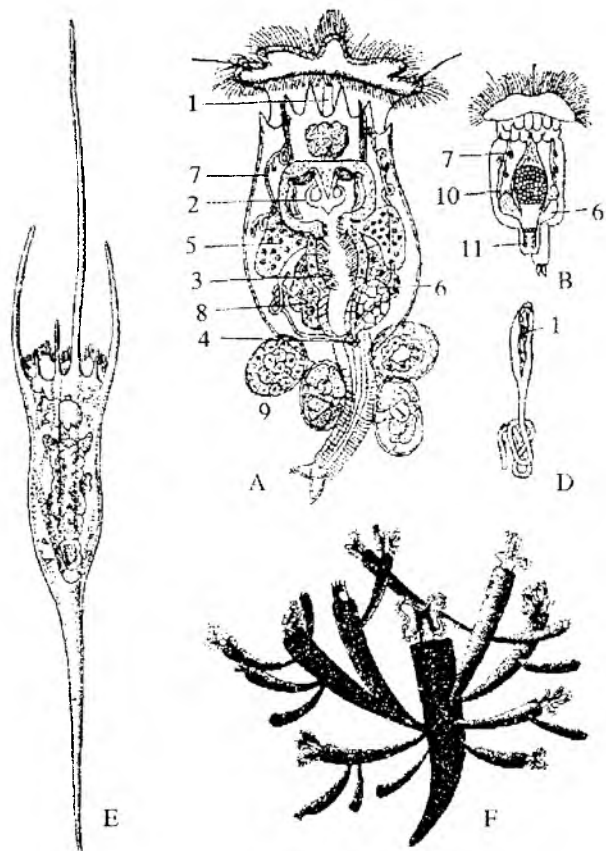
74-rasm. Og'izaylangichlilar. A, B, D – Branchionus urceolaris (A – urg'ochi, B – erkak, D – protonefridiy), E – plankton Notholca longispina , F – o'troq Melicerta ringens (individlar bir-birining himoya nayiga yopishib olgan): 1 – paypaslagich, 2 – mastaks, 3 – “oshqozon”, 4 – orqa chiqaruv teshigi, 5 – so'lak bezi, 6 – qovuq, 7 – protonefridiy, 8 – tuxumdon, 9 – tuxum, 10 – urug'don, 11 – kuyikish organi.
