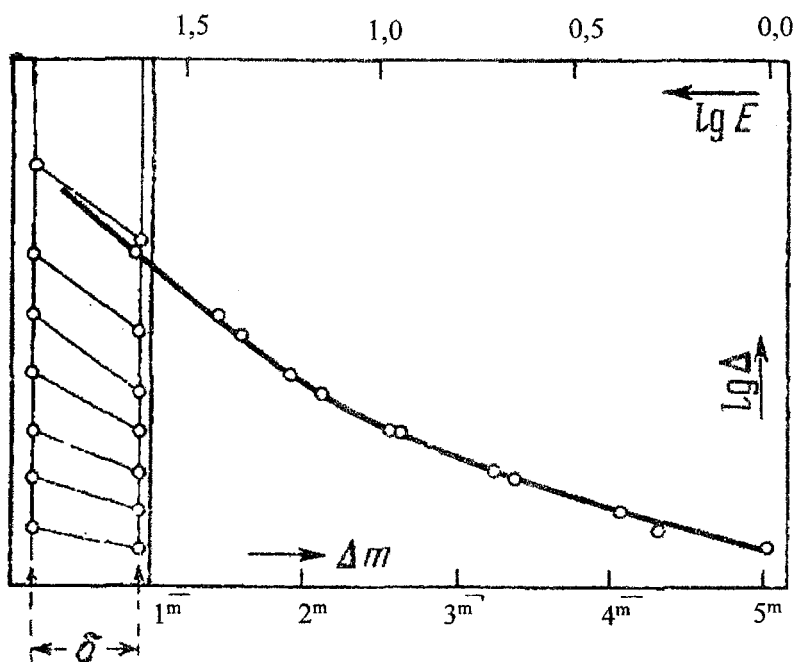
6-rasm. Spektrogramma uchun kalibrovka egri chizig'ini tuzish.
