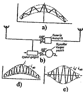
18-rasm. Interferometrlar ishlash tamoyli
