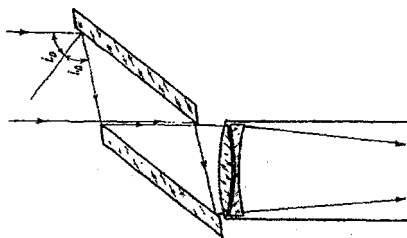
45-rasm. Marblit ko'zgusini polyarizatsion o'rnatish.
