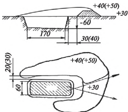
50-siwret. Avtomattan dizerlep otirip atiw usin okop.
